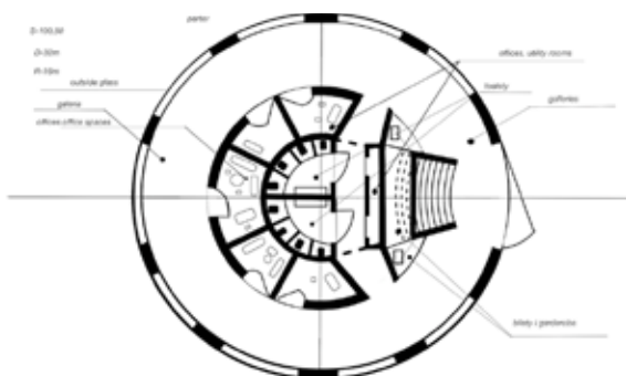
Parter
